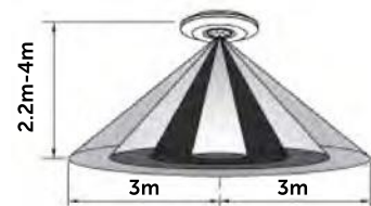
Installation Height: 2.2m-4m
